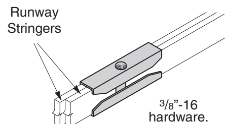
SB166B For Dual Stringers
