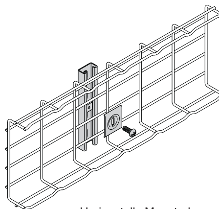
Horizontally Mounted
