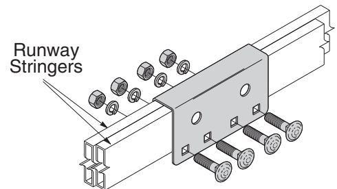
SB168D For Dual Stringers
