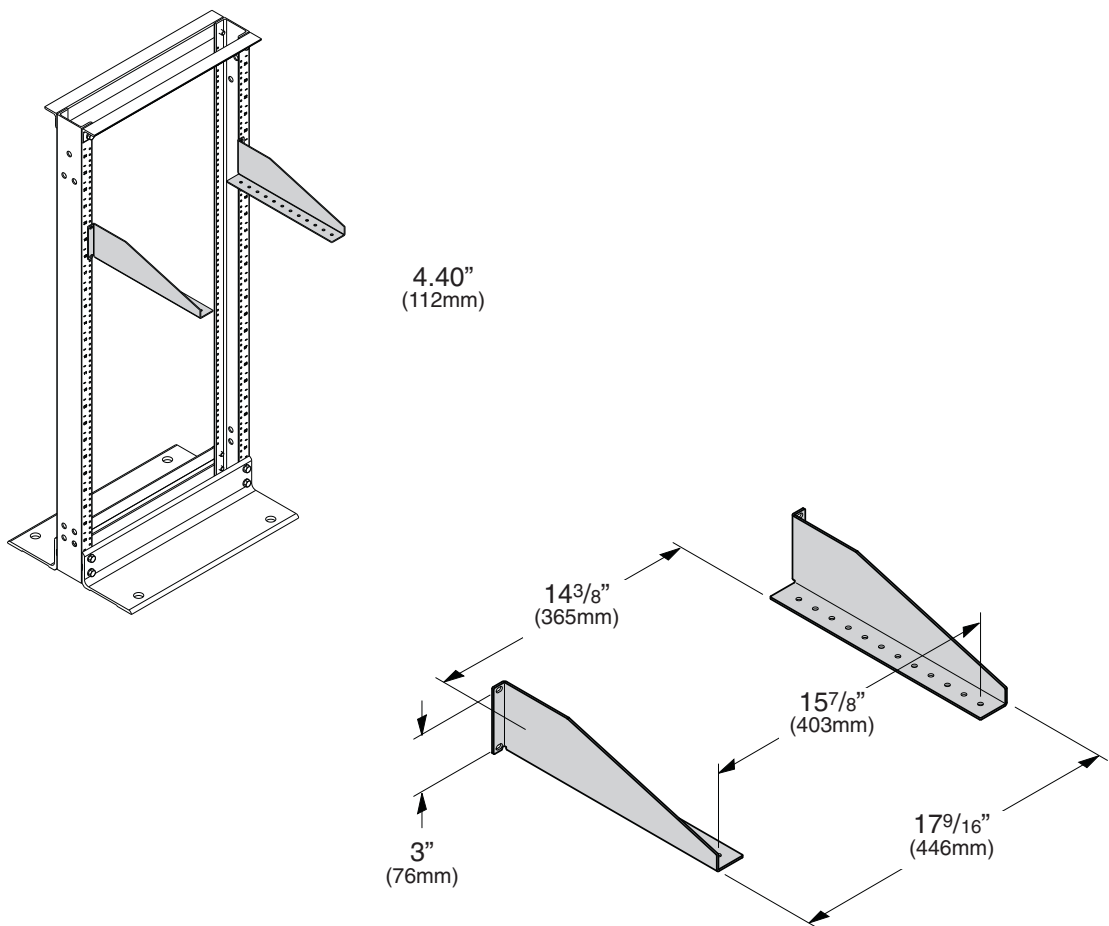
Equipment Support Bracket
