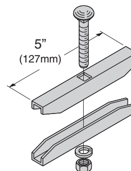
SB166A For Single Stringer
