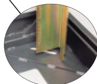
Heavy Duty Corner Construction Extra welded gusset plates maintain cabinet integrity in seismic situations.
